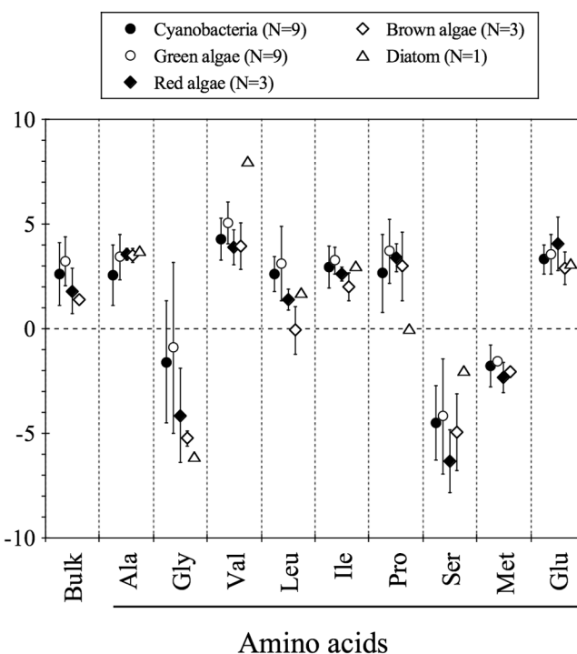
Fig. 4. \beta Patterns for photoautotrophs. Symbols and bars represent the means and variations ( 1\sigma ) of the \beta values for a single taxon of primary producers.
