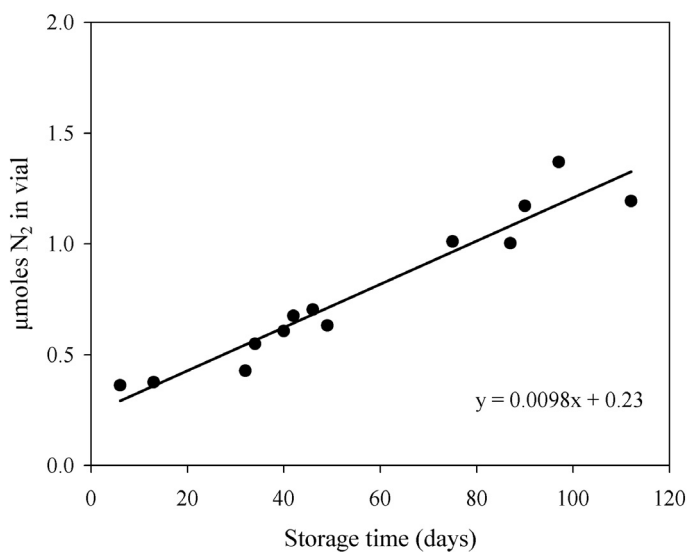
Fig. 2. Change in N 2 content in re-evacuated Exetainer vials during storage in water
