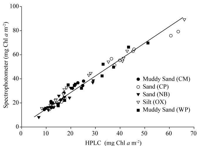
Fig. 6. Simple linear regression of BMA biomass of differing sediment types using spectrophotometry and HPLC ( n = 66 ). Line indicates regression slope (spectrophotometer = 2.877 + 1.329 * \text{HPLC} , r^2 = 0.96 ).
