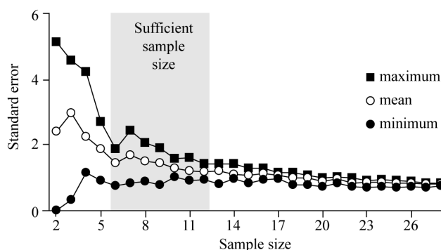
Fig. 5. Assessment of required sample number for determining benthic microalgal abundance at the meters squared scale (Day and Quinn 1998). Samples from Moreton Banks.
