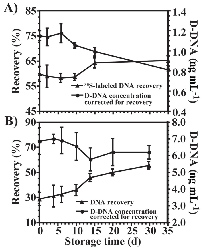
Fig. 5. Effect of storage time on recovery of ^{35}\text{S} -labeled DNA and D-DNA concentration corrected for ^{35}\text{S} -labeled DNA recovery in 0.22 \mu m-filtered seawater samples (A). Effect of storage time on recovery of lambda phage DNA internal standards in replicate samples and D-DNA concentrations corrected for DNA internal standard recovery in 0.22 \mu m-filtered seawater samples (B). Error bars represent one standard deviation of the mean ( n = 4 ).
