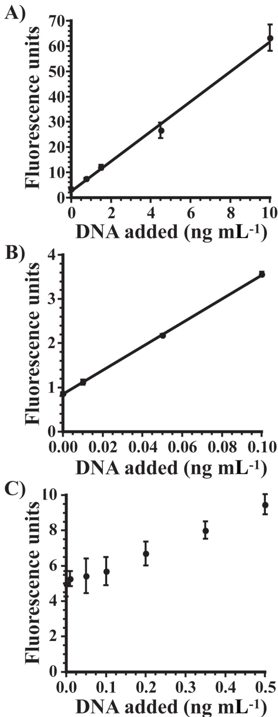
Fig. 4. Internal standard curve of lambda phage DNA added to 0.22 \mu m-filtered seawater with DNase (Sigma-Aldrich #D7291) and analyzed using the centrifugal concentration method (A). Determination of the detection limit of the centrifugal concentration method with DNase (Sigma-Aldrich #D7291) addition (B) and lower-grade DNase (Sigma-Aldrich #D5025) addition (C) using lambda phage DNA added to 10 kDa-filtered seawater. Error bars represent one standard deviation of the mean ( n = 3 ). The r^2 values for the regression lines (A and B) are > 0.99 .
