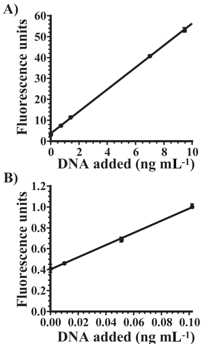
Fig. 3. Internal standard curve of lambda phage DNA added to 0.22 μm-filtered seawater (A) and determination of the detection limit of the centrifugal concentration method using lambda phage DNA added to 10 kDa-filtered seawater (B). Error bars represent one standard deviation of the mean ( n = 3 ). The r^2 values for the regression lines (A and B) are > 0.99 .
