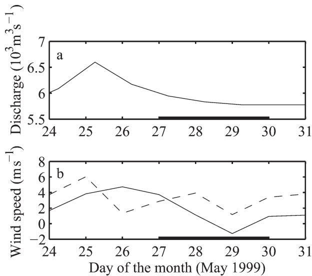
Fig. 2. Niagara River discharge and local wind, 24–31 May 1999. (a) Discharge, measured at the head of the river, shifted by 18 h to account for the propagation time in the river. (b) Wind speed measured at St. Catherines airport. Solid line: alongshore wind; dashed line: cross-shore wind. In panels a and b the solid bar on the time axis corresponds to the study period.
