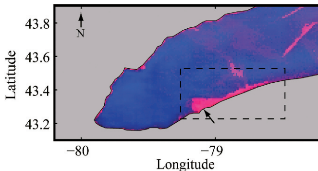
Fig. 4. Surface temperature at 18:30 h coordinated universal time on 29 May 1999 from advanced very-high-resolution radiometer sensor. The plume and ambient lake temperatures are approximately 12°C and 6°C. The diffuse regions of higher temperature to the north and east of the plume are most likely the result of thin cloud cover. The rectangle shows the approximate boundary of the SeaWiFS images in Fig. 3 and the arrow shows the location of the river mouth.
