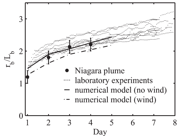
Fig. 6. Comparison of satellite data from the Niagara River plume to laboratory and numerical model studies. The laboratory data are from Horner-Devine et al. (2006), and include 13 experiments spanning a large range of Rossby and Froude numbers. The numerical data were obtained using the same model (ECOM3D) as Fong and Geyer (2002) with inflow parameters set to those of the Niagara River during the period 27 to 30 May 1999 with and without wind forcing. Error bars for the satellite data are \pm 0.5 km, on the basis of the nominal SeaWiFS sensor resolution of 1 km.
