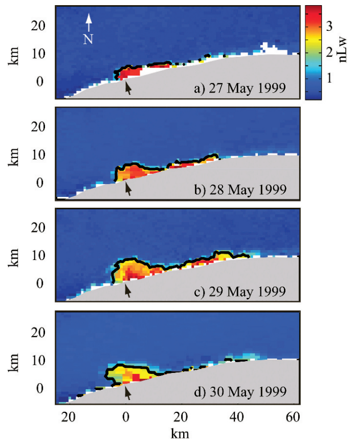
Fig. 3. Normalized water-leaving radiance showing the Niagara River plume on (a) 27 May 1999, (b) 28 May 1999, (c) 29 May 1999, and (d) 30 May 1999. The color corresponds to normalized water-leaving radiance (nLw) in units of \text{mW cm}^{-2} \mu\text{m}^{-1} \text{sr}^{-1} . The black contour indicates the threshold chosen to represent the edge of the plume and the Niagara River mouth is indicated by the black arrow. White cells near the shoreline are bad data.
