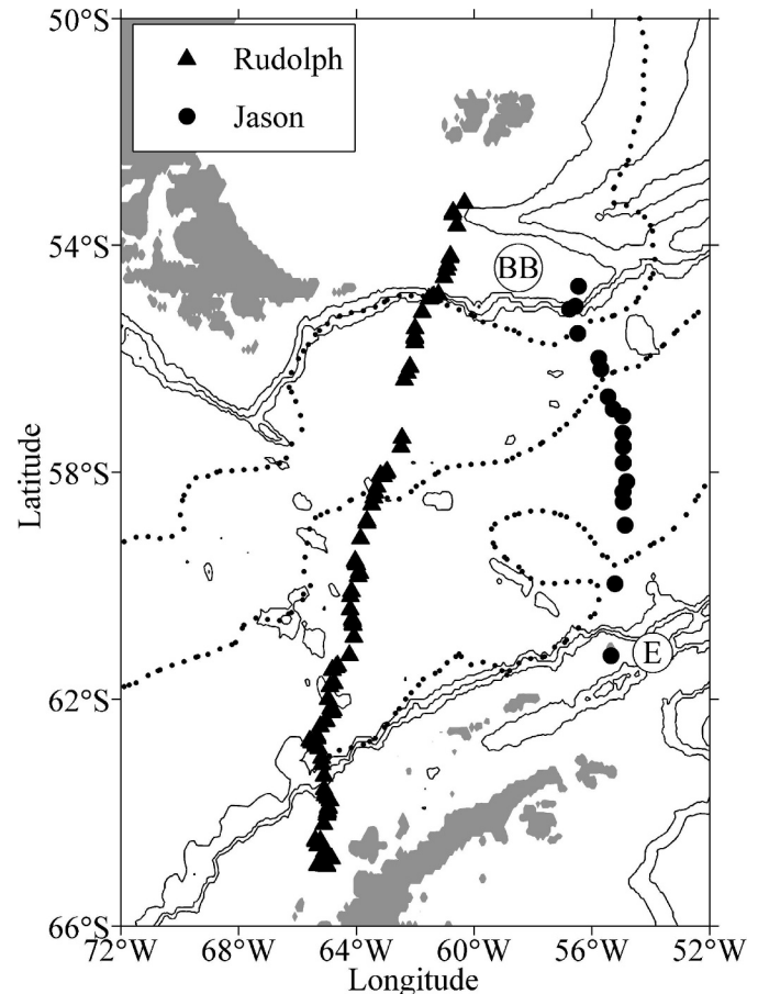
Fig. 1. The positions of the CTD-SRDL hydrographic profiles from Rudolph (triangles) and Jason (circles) sampled 07–20 June 2004 and 01–15 April 2005 respectively. The mean position for 2004 and 2005 of the Subantarctic Front, Polar Front, and southern ACC Front (from north to south) by Boehme et al. (in press) are shown as dotted lines. Burdwood Bank (BB) and Elephant Island (E) are marked. Isobaths are 1,000 m, 2,000 m, and 3,000 m and land is shaded gray.
