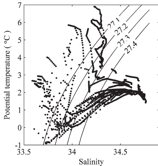
Fig. 4. Potential temperature versus salinity for the stations made by Jason. The \sigma_{\theta} = 27.3 \text{ kg m}^{-3} isopycnal marks the approximate density of the Antarctic Intermediate Water of the Drake Passage.
