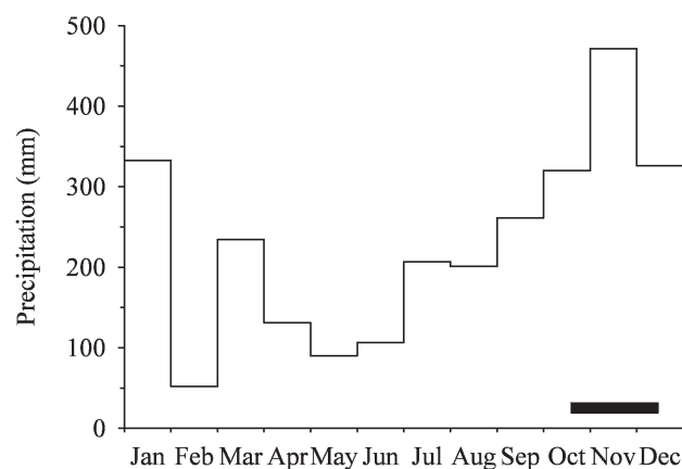
Fig. 2. Average monthly precipitation at CALTEX Meteorological Station, Dumai airport, in 2003. The black bar denotes the sampling period from 13 October to 15 December 2003.
