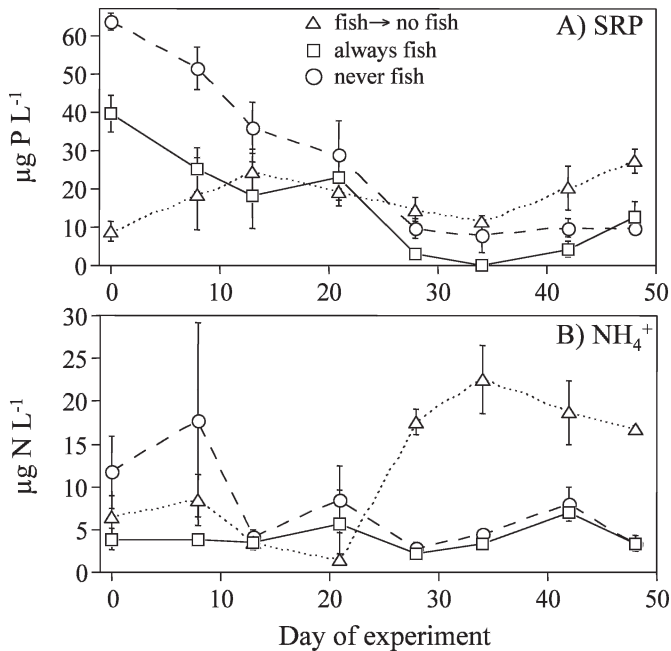
Fig. 4. Dynamics of (A) SRP and (B) NH 4 + during Phase 2 of the experiment. Error bars represent 1 SE.
