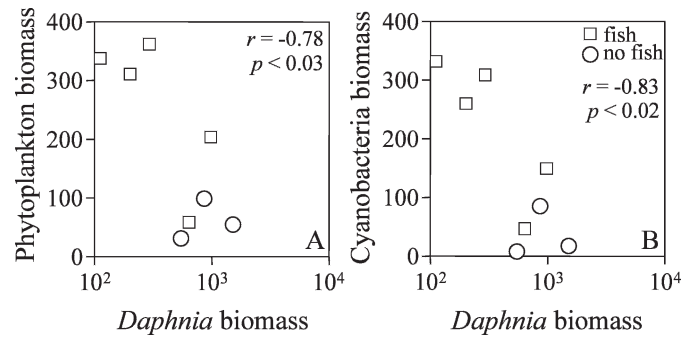
Fig. 1. Relationships between Daphnia biomass ( \mu\text{g dry mass L}^{-1} ) and the biomass ( \mu\text{g dry mass L}^{-1} ) of (A) phytoplankton and (B) cyanobacteria (mixture of Anabaena flos-aquae and Microcystis aeruginosa ) at the end of Phase 1 of the experiment (day 0 of Phase 2). Squares, enclosures with fish; circles, enclosures lacking fish. Statistics refer to linear correlations of y versus \log_{10}x .
