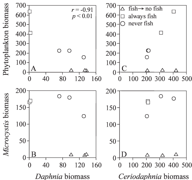
Fig. 6. Relationships between Daphnia biomass ( \mu\text{g dry mass L}^{-1} ) and the biomass ( \mu\text{g dry mass L}^{-1} ) of (A) phytoplankton and (B) Microcystis aeruginosa , and between Ceriodaphnia biomass and the biomass of (C) phytoplankton and (D) M. aeruginosa at the end of Phase 2 of the experiment. Each data point represents biomass averaged over the last three sampling dates (days 34–48) for each of eight enclosures (two with fish, six without fish). Statistics refer to linear correlations.
