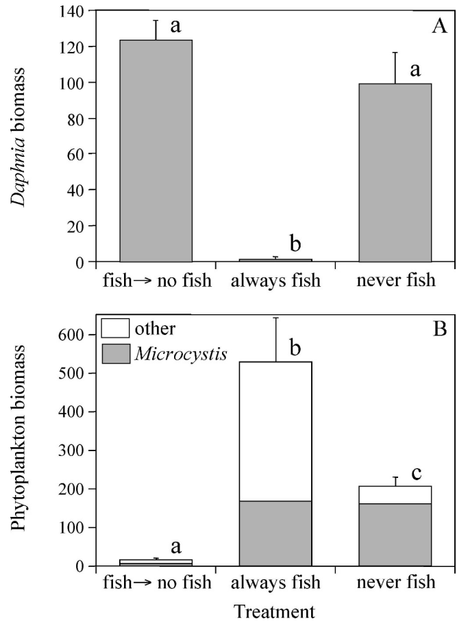
Fig. 5. Mean biomass (µg dry mass L -1 ) of (A) Daphnia and (B) phytoplankton over the last three sampling dates of the experiment. Ceratium hirundinella dominated the “other” category in the always-fish treatment. Error bars represent 1 SE. Significantly different means (Tukey-Kramer HSD, p < 0.05) are indicated with different lowercase letters.
