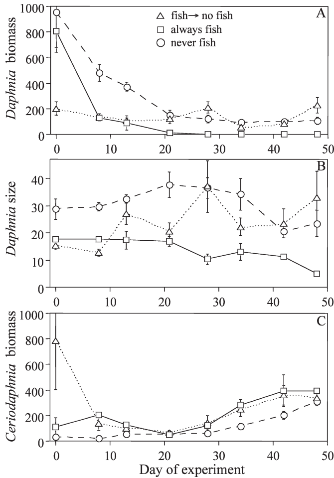
Fig. 2. Dynamics of (A) Daphnia biomass ( \mu\text{g dry mass L}^{-1} ), (B) Daphnia individual size ( \mu\text{g} ), and (C) Ceriodaphnia biomass ( \mu\text{g dry mass L}^{-1} ) during Phase 2 of the experiment. Error bars represent 1 SE.
