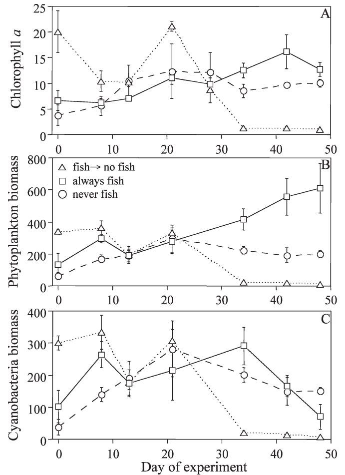
Fig. 3. Dynamics of (A) Chl a ( \mu\text{g L}^{-1} ), (B) total phytoplankton biomass ( \mu\text{g dry mass L}^{-1} ), and (C) total cyanobacteria biomass ( \mu\text{g dry mass L}^{-1} ) during Phase 2 of the experiment. Error bars represent 1 SE.
