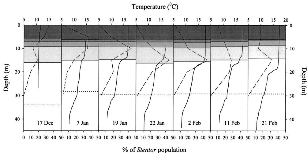
Fig. 1. Vertical profiles of the relative abundance of S. araucanus (dashed line), temperature (solid line) and depth of 1% of surface PAR (dotted line), and UV (305, 320, 340, and 380 nm, gray scale) in Lake Moreno Oeste during summer 2003–2004.
