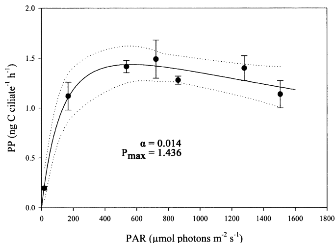
Fig. 5. Laboratory P/E curve of S. araucanus . Dotted line represents 95% confidence limits.
