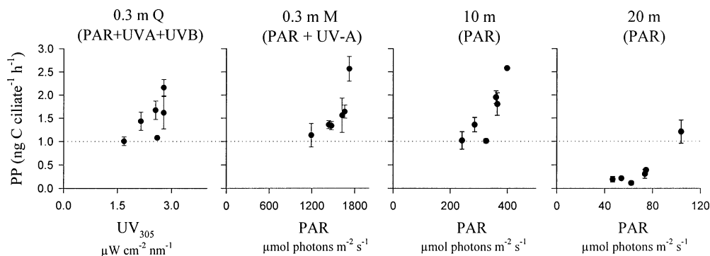
Fig. 3. Primary production in S. araucanus in relation to UV-B (305 nm) and PAR wavelengths during static incubations (Q: quartz tubes for full sunlight; M: quartz tubes wrapped with Mylar ® ). Dotted line represents the level of 1 ng C ciliate -1 h -1 .
