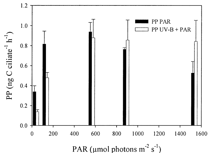
Fig. 6. Primary production of S. araucanus in laboratory experiments carried out with acclimatized organisms (15 h exposure to UV-B+PAR and PAR).
