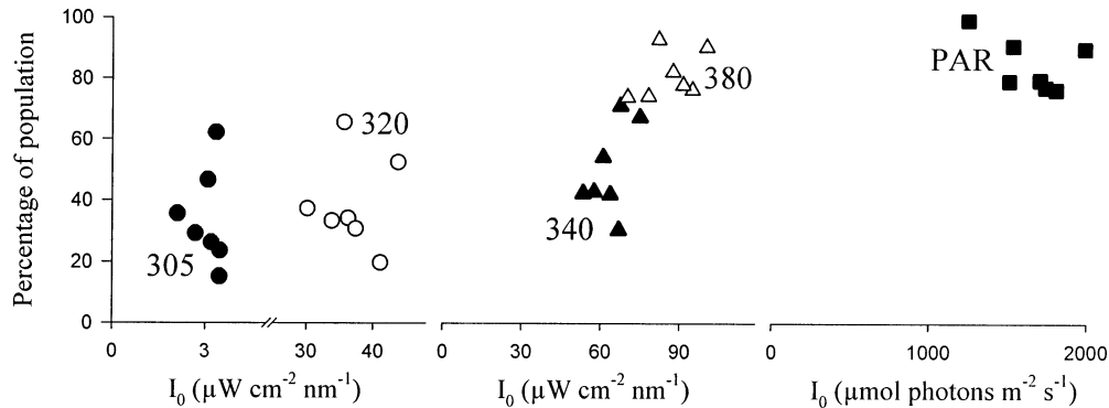
Fig. 2. Percent of S. araucanus population (as an integration of abundances from 0 to Z_{1\%} of the corresponding wavelength) exposed to more than 1% of surface irradiance ( I_0 ) of the different wavelengths (filled circles: 305 nm; open circles: 320 nm; filled triangles: 340 nm; open triangles: 380 nm; and squares: PAR).
