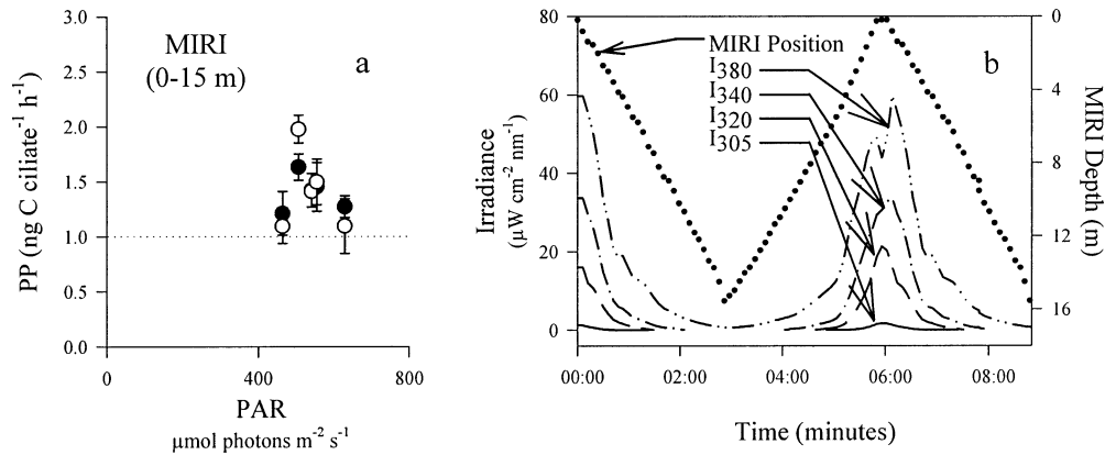
Fig. 4. (a) Primary production in S. araucanus during the epilimnetic variable-depth incubations (MIRI) from 0 m to 15 m in depth. Filled circles: quartz tubes for full sunlight; and open circles: quartz tubes wrapped with Mylar ® . Light intensity was calculated according to Helbling et al. (1994). Dotted line as in Fig. 3. (b) UVR received in a simulated cycle of the MIRI, measured with the PUV 500B.
