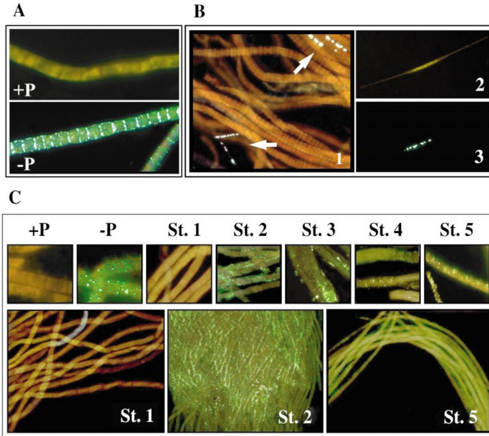
Fig. 1. (A) ELF-assayed phosphorus-replete (+P) and phosphorus-stressed (-P) T. erythraeum controls imaged with a DAPI long-pass filter set. Phycoerythrin autofluorescence is visible in the +P cells, whereas the green fluorescent product is PhoA-cleaved ELF. (B) Analyses of the specificity of the ELF reaction. (1) P-replete Trichodesmium samples (not ELF-labeled) from Sta. 1 associated with Plectonema sp. (arrows) that do have PhoA activity (ELF-labeled). (2) Phycoerythrin fluorescence in Plectonema from Sta. 1 observed by use of the Rhodamine filter set. (3) The same cell when viewed with a DAPI long-pass filter set to detect the fluorescent ELF product. (C) Culture controls and field populations of Trichodesmium from the western North Atlantic assayed for PhoA activity with ELF. Thumbnail images (top panel) of ELF-assayed trichomes are from +P and -P culture controls as well as stations (1–5) along a November 2000 cruise track. P-stressed cells are evident due to the PhoA-generated green fluorescent ELF precipitate. Phycoerythrin autofluorescence is also visible. In the bottom panel, larger images of representative colonies are shown for Sta. 1 (no ELF labeling), 2 (ELF-labeled), and 5 (ELF-labeled), respectively.
