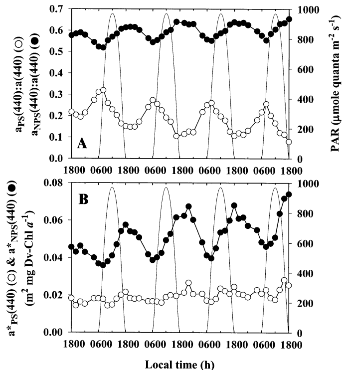
Fig. 5. Temporal variations of the absorption properties of Prochlorococcus PCC 9511 grown in a cyclostat. (A) Relative proportion of photosynthetic and nonphotosynthetic absorption. (B) Dv-Chl a specific absorption coefficient at 440 nm for photosynthetic and nonphotosynthetic pigments.
