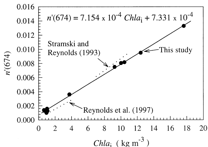
Fig. 10. The imaginary part of the refractive index n' at 674 nm as a function of the intracellular Chl a concentration \text{Chl } a_i for T. pseudonana grown under various conditions. Twelve data points for which Chl a was determined by HPLC (see text for more details) and the regression line with the corresponding equation are shown. The squared correlation coefficient is 0.998. The data points having the lowest values of the variables represent temperature and nitrogen limitation, the five data points with the highest values are for light limitation, and the intermediate point is for optimal growth conditions. For comparison, the relationships obtained previously for the same species by Stramski and Reynolds (1993) and Reynolds et al. (1997) are also shown (dotted lines).
