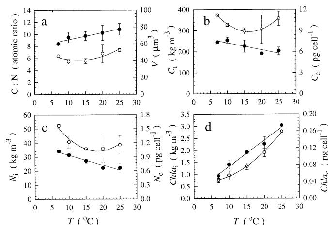
Fig. 3. The responses of cellular properties to variations in temperature for T. pseudonana grown under saturating light and nutrient-replete conditions. (a) Carbon-to-nitrogen ratio, C:N (solid circles), and mean cell volume, V (open circles). (b) Carbon content per cell, C_c (open circles), and intracellular concentration of carbon, C_i (solid circles). (c) Nitrogen content per cell, N_c (open circles), and intracellular concentration of nitrogen, N_i (solid circles). (d) Chl a content per cell, Chl a c (open circles), and intracellular concentration of Chl a , Chl a i (solid circles). The Chl a values for intermediate temperatures were derived from the imaginary part of the refractive index (see text and Fig. 10 for details). The average value and standard deviation is shown for each variable at each temperature. The data points are accompanied by trend lines.
