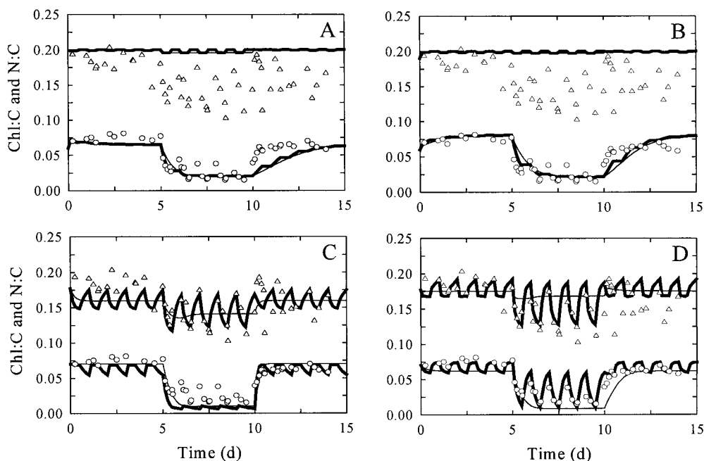
Fig. 3. Comparisons of model output with experimental data for N:C (triangles) and Chl:C (circles); cf. Fig. 2. Panels present model output from (A) GM1, (B) GM2, (C) FM1, and (D) FM2. Thin lines are for simulations where light was supplied continuously to attain the daily photon dose. Thick lines are for simulations where light was supplied in a 12 h:12 h light:dark cycle, as used in the experiments.
