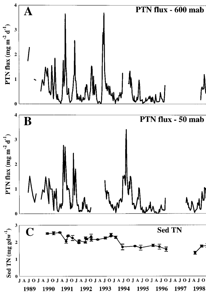
Fig. 3. (A) PTN flux measured with sediment traps moored at Sta. M at 600 mab. Gaps in the data set of <30 d are connected by linear interpolation; gaps of >30 d are depicted as breaks in the record with no interpolation between data points. (B) PTN flux measured with sediment traps moored at Sta. M at 50 mab. Gaps are represented as in panel A. (C) Mean, maximum, and minimum concentration of total nitrogen (SedTN) in the uppermost 10 mm of the sediments. Each value calculated as the mean of concentrations from sediment sections taken at 2.5-mm intervals below the sediment surface (four sections). Symbols represent empirical measurements of sediment total nitrogen concentrations. Lines connecting means are the result of linear interpolation between data points.
