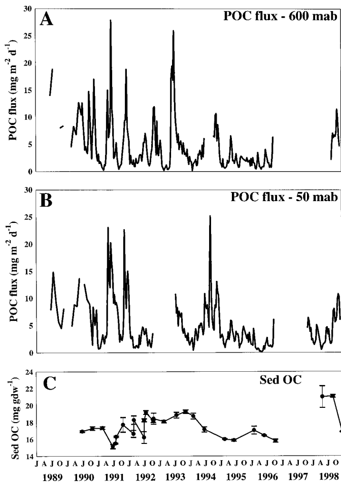
Fig. 2. (A) POC flux measured with sediment traps moored at Sta. M at 600 mab. Gaps in the data set of <30 d are connected by linear interpolation; gaps of >30 d are depicted as breaks in the record with no interpolation between data points. (B) POC flux measured with sediment traps moored at Sta. M at 50 mab. Gaps are represented as in panel A. (C) Mean, maximum, and minimum concentration of organic carbon (SedOC) in the uppermost 10 mm of the sediments. Each value calculated as the mean of concentrations from sediment sections taken at 2.5-mm intervals below the sediment surface (four sections). Symbols represent empirical measurements of sediment organic carbon concentrations. Lines connecting means are the result of linear interpolation between data points.
