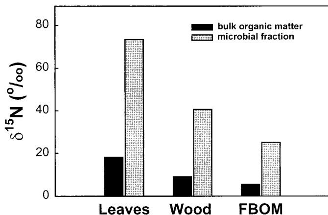
Fig. 8. Comparison of \delta^{15}\text{N} values of bulk allochthonous organic matter vs. the microbial N associated with the organic matter/microbe complex on day 38. \delta^{15}\text{N} values are plotted for leaves, wood, and FBOM at the 50-m site.
