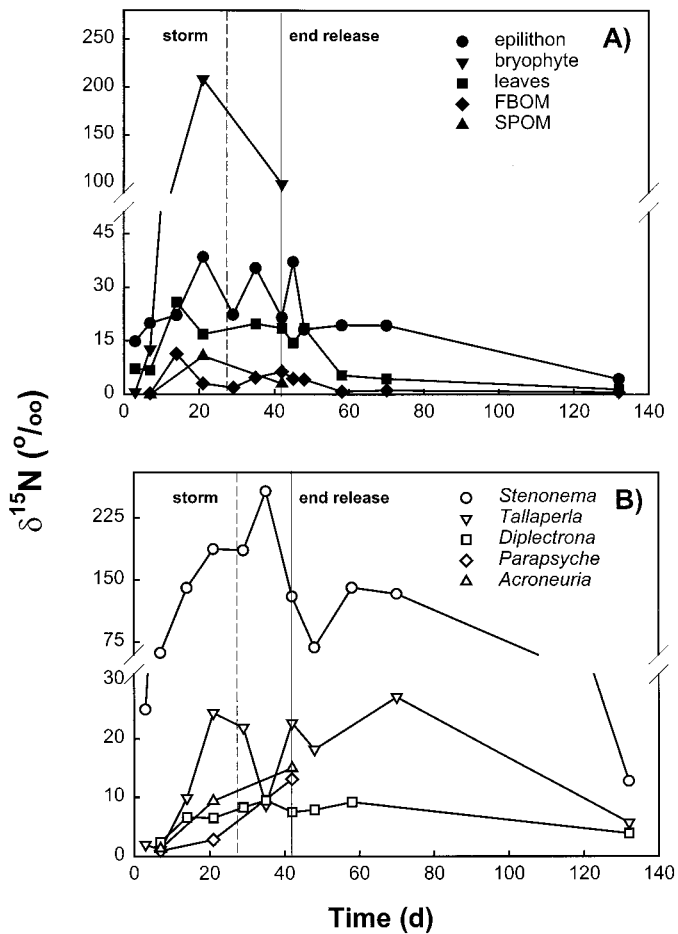
Fig. 5. Time series of observed \delta^{15}\text{N} values at 27 m for the (A) primary uptake compartments, and (B) consumers. The dotted line marks the storm on day 27 and the solid line marks the end of the tracer addition on day 42.
