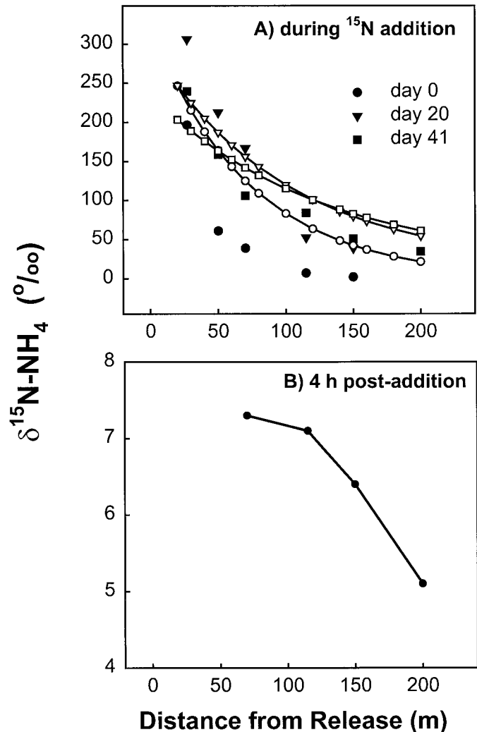
Fig. 2. (A) Longitudinal profile of observed (solid symbols) vs. predicted (open symbols) decline in \delta^{15}\text{N-NH}_4 on days 0, 20, and 41 of the tracer addition. (B) Observed longitudinal profile of \delta^{15}\text{N-NH}_4 4 h after the tracer addition stopped on day 42.
