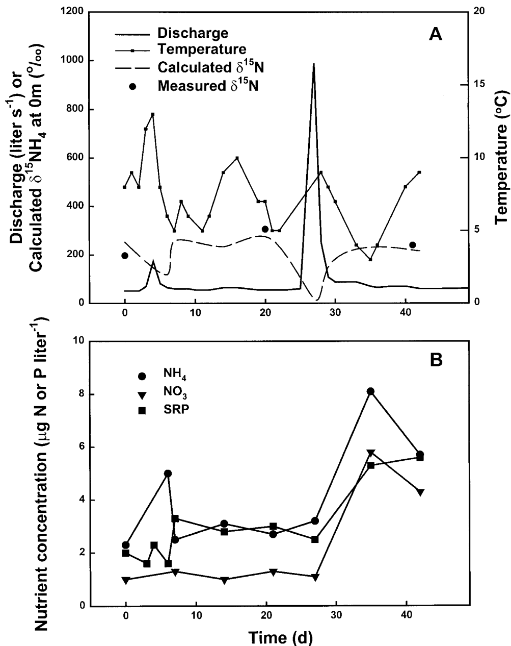
Fig. 1. (A) Discharge, stream temperature, calculated \delta^{15}\text{NH}_4 at 0 m, and measured \delta^{15}\text{NH}_4 at 27 m during the tracer addition. Calculated \delta^{15}\text{NH}_4 values are based on daily discharge, weekly stream ammonium concentrations, and daily drip rate of the release solution of \delta^{15}\text{NH}_4\text{Cl} . (B) Concentrations of ammonium, nitrate, and soluble reactive phosphorus measured approximately weekly during the tracer addition.
