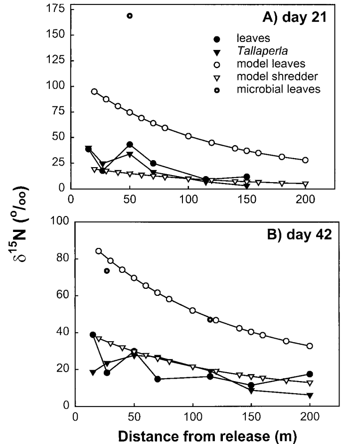
Fig. 6. Longitudinal profile of observed (solid symbols) vs. predicted (open symbols) decline in \delta^{15}\text{N} values of leaves and the shredding stonefly Tallaperla on (A) day 21 and (B) day 42 of the tracer addition. Microbial ^{15}\text{N} value for leaves is also plotted for reference (crossed solid circle).
