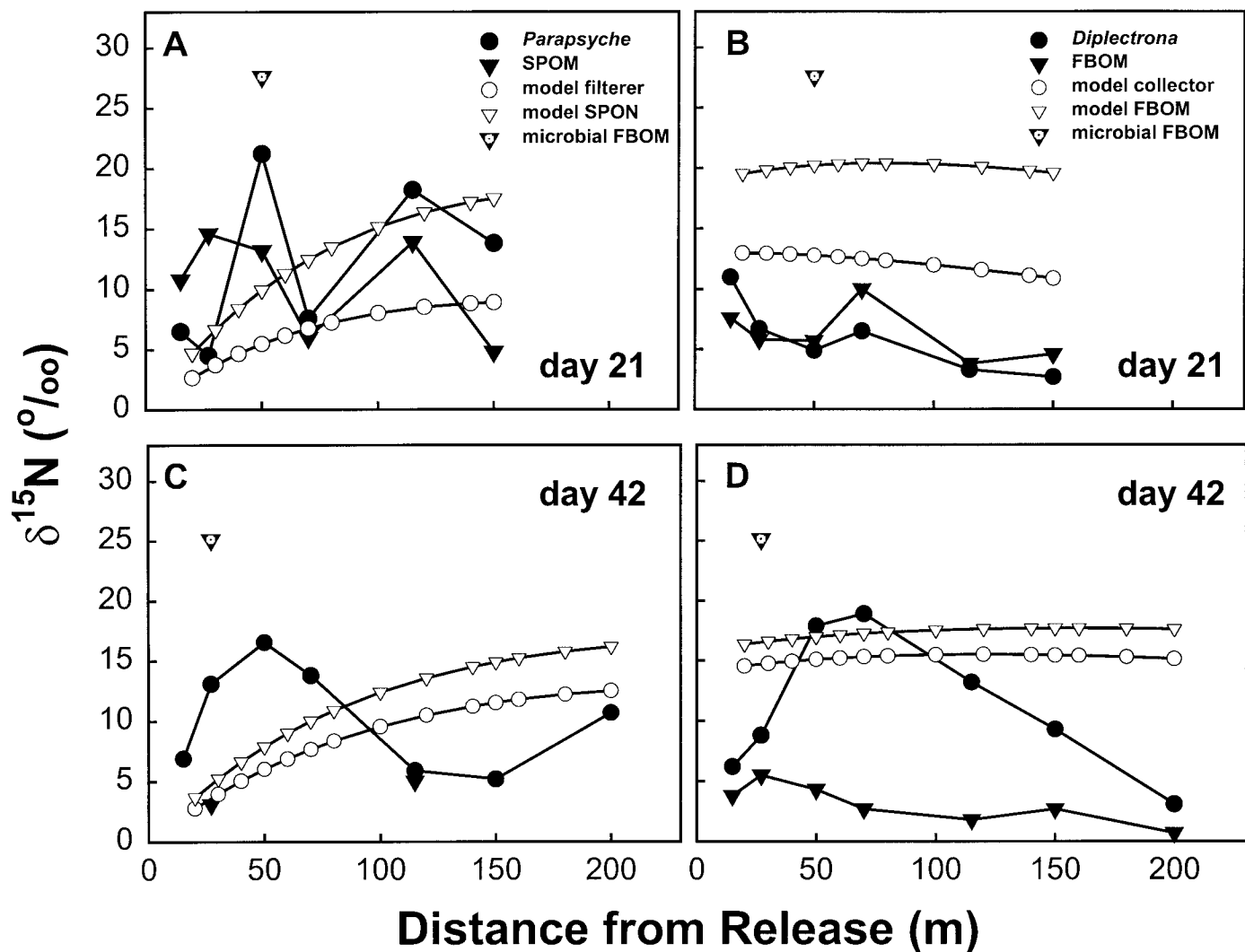
Fig. 7. Comparison of suspended vs. benthic particle pathways. Longitudinal profile of observed (solid symbols) vs. predicted (open symbols) decline in \delta^{15}\text{N} values of (A) the filtering caddisfly Parapsyche and seston on day 21 and (C) day 42 of the tracer addition. Similar plots of the longitudinal profile of the collecting caddisfly Diplectrona and FBOM on (B) day 21 and (D) day 42 of the tracer addition. Microbial ^{15}\text{N} value for FBOM is plotted for reference (crossed solid triangle).
