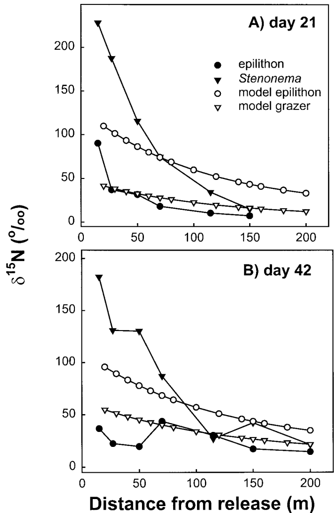
Fig. 4. Longitudinal profile of observed (solid symbols) vs. predicted (open symbols) decline in \delta^{15}\text{N} values of epilithon and the grazing mayfly Stenonema on (A) day 21 and (B) day 42 of the tracer addition.
